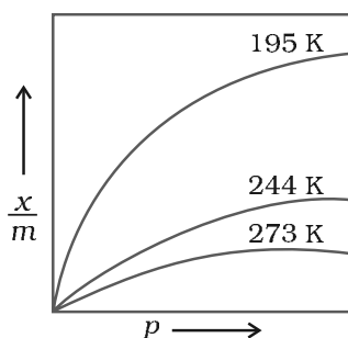
Fig. 5.1: Adsorption isotherm
