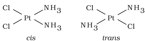
Fig. 9.2: Geometrical isomers ( cis and trans ) of \text{Pt}(\text{NH}_3)_2\text{Cl}_2
